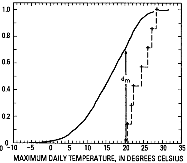
Figure 42.--Probability distribution functions for daily maximum temperature measured at Paradise Ranger Station, Mount Rainier, for months May through November in the years 1986 through 1992, including only rainless days.
