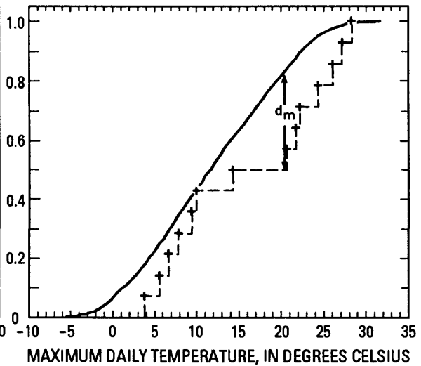
Figure 40.--Probability distribution functions for daily maximum temperature measured at Paradise Ranger Station, Mount Rainier, for months May through November in the years 1986 through 1992.
