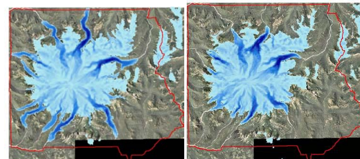
Figure 50 cont'd. Spatial extents of Holocene Glaciers on Mount Rainer for Model 1 and 2. 160-5,520 cal yr. B.P. are modeled with the current DEM. For Model 1 years 7,490-11,490 cal yr. B.P. are modeled with a DEM representing a taller Mount Rainer before the Osceola lahar 5,600 cal yr. B.P. Model 2 uses the current DEM throughout.
