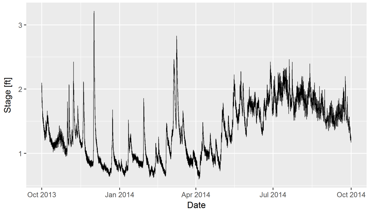
Figure 3: Stream stage during water year 2014 at Longmire.
