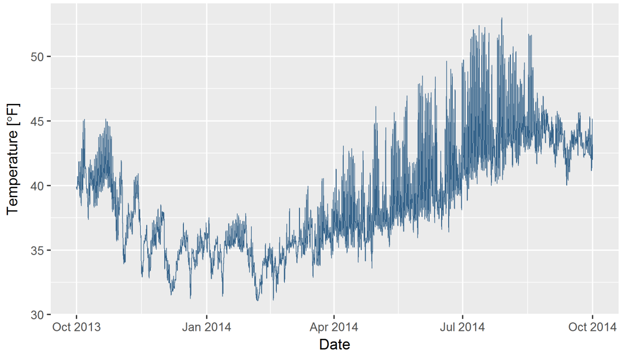
Figure 4: Stream temperature during water year 2014 at Longmire.
