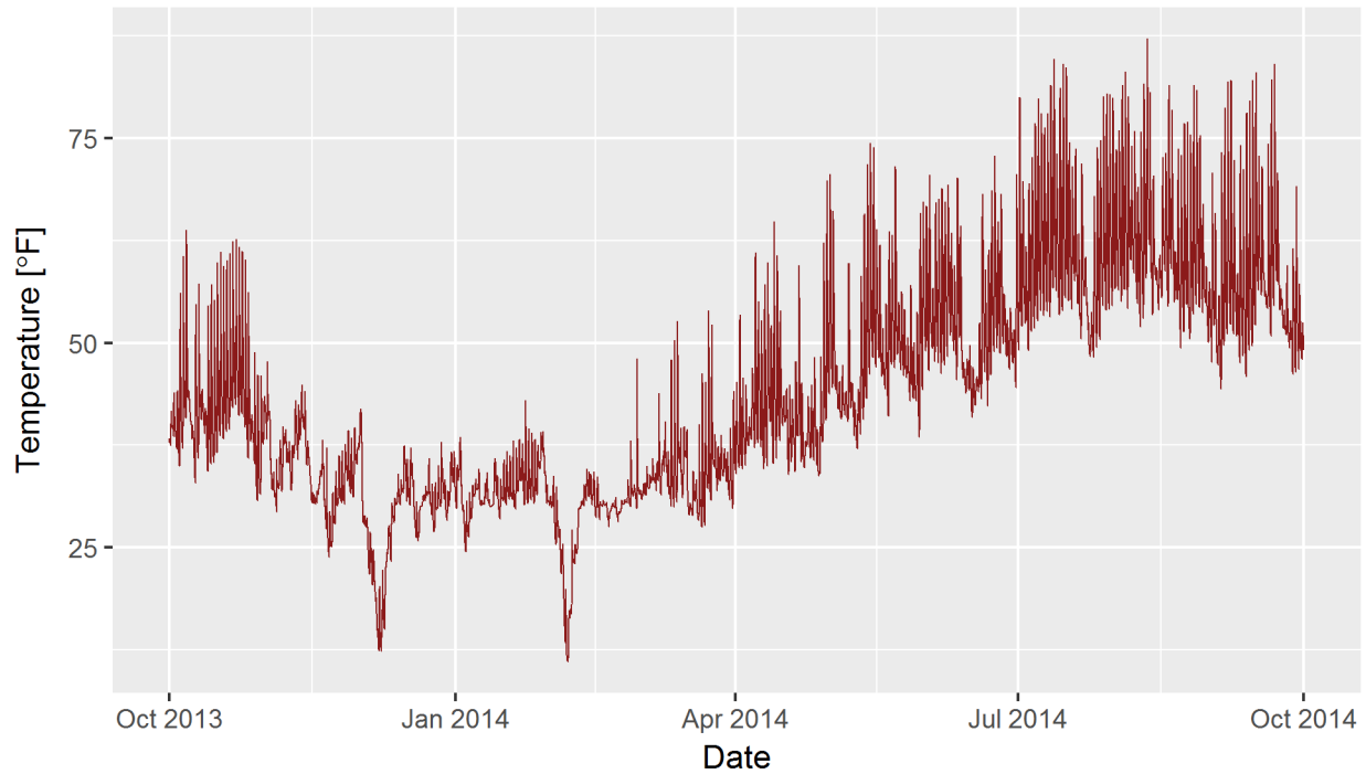
Figure 5: Air temperature during water year 2014 at Longmire.
