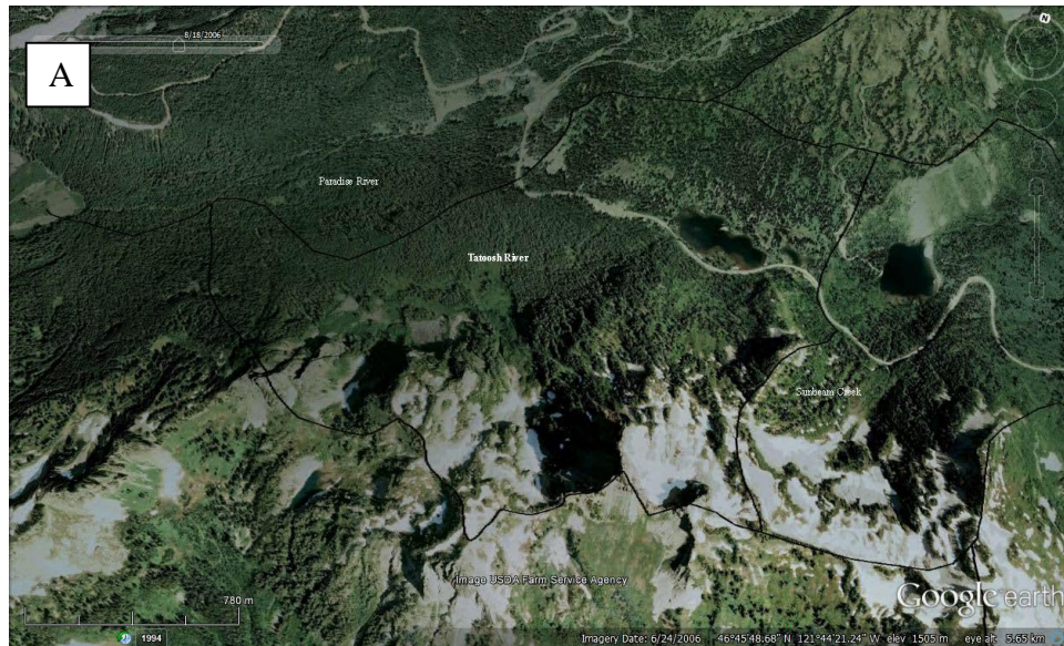
Figure 65. a) Google Earth image of Tatoosh Drainage in August 2006.
