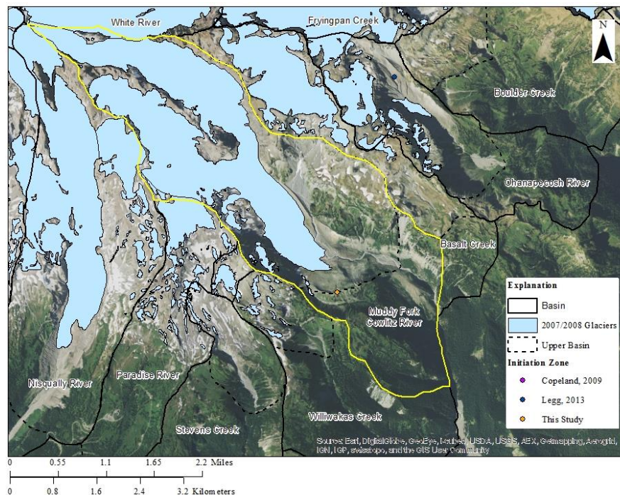
Figure 30. Muddy Fork Cowlitz basin outlined in yellow, other basins outlined in black, the upper basin outlined in dashed black, glaciers in blue.
