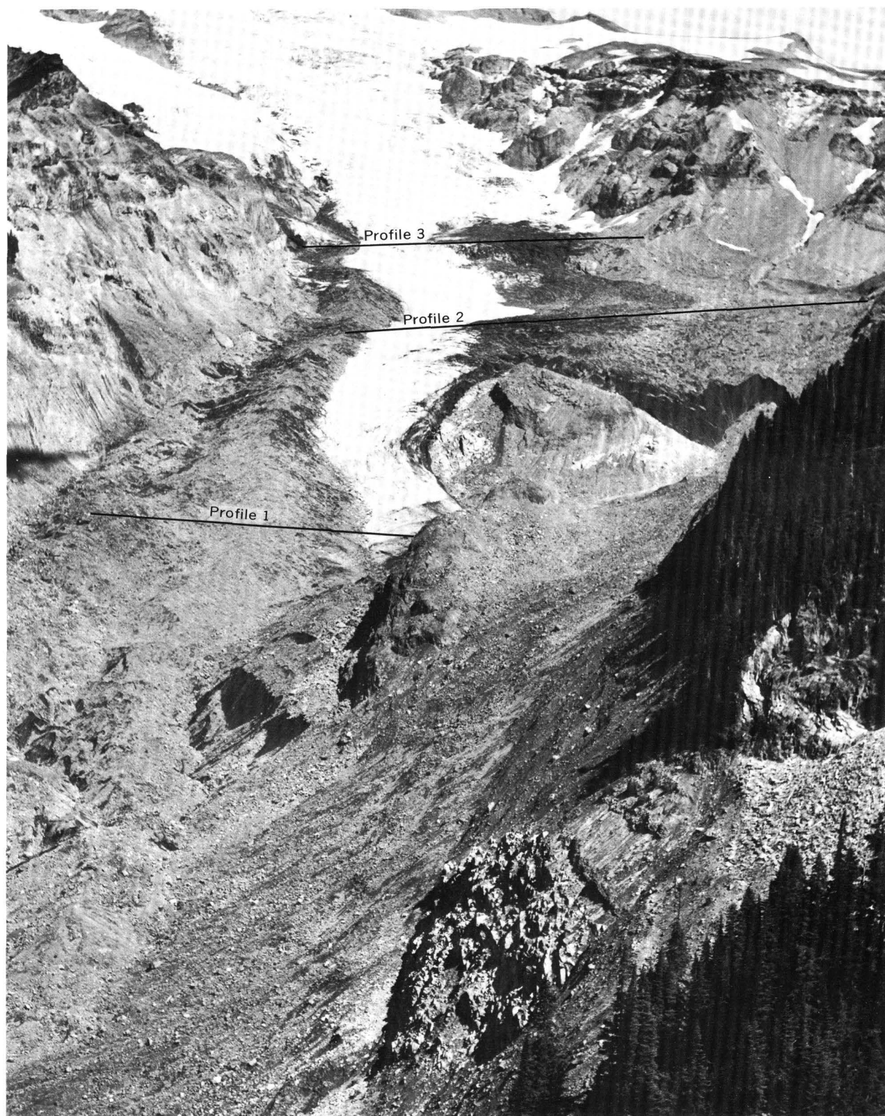
Figure 20.—Lower part of Nisqually Glacier as seen from station 5 on August 31, 1942. Approximate locations of the surveyed cross profiles are shown. Entire glacier is receding. Area down glacier from profile 1 (lower end of the white ice) is stagnant, as indicated by hummocky, debris-covered, noncrevassed ice. Note the long morainelike ridge of debris-covered ice immediately to left of the white ice. The nunatak is bare. Note debris load on right half of the glacier from profile 3 downstream.
