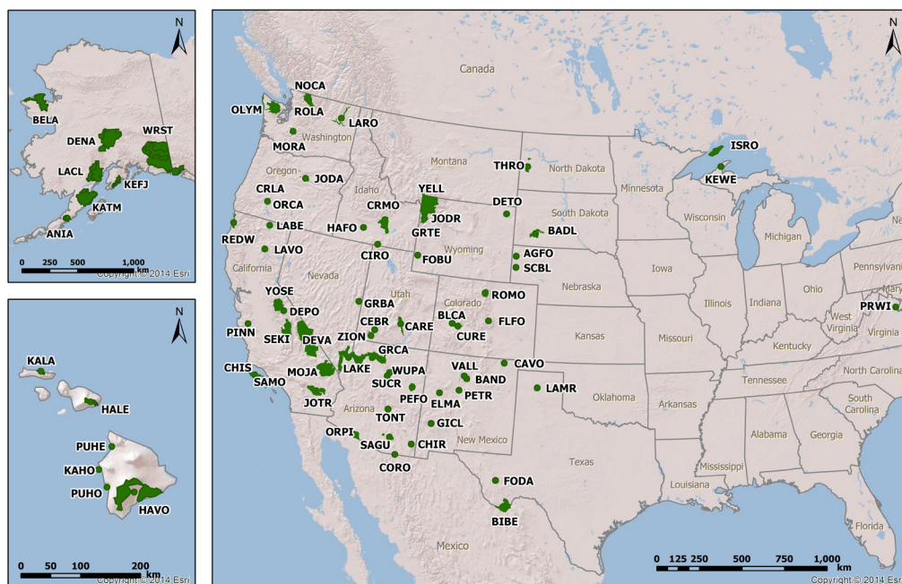
Figure 1. Map of national parks and monuments that contain volcanoes or volcanic deposits. Parks are labeled with NPS 4-letter abbreviations, for a description of these units and their full names see Table 2. Not pictured: National Park of American Samoa (NPSA) and Virgin Islands National Park (VIIS)
