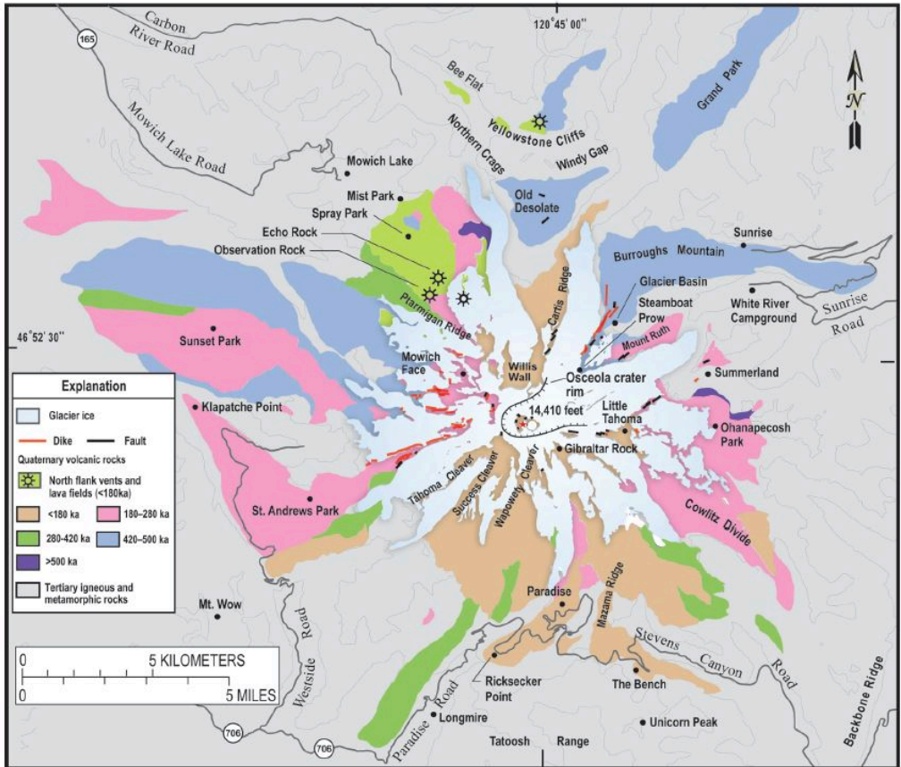
Figure 5. Simplified geologic map of Mount Rainier. USGS figure modified from Driedger et al., 2005.
