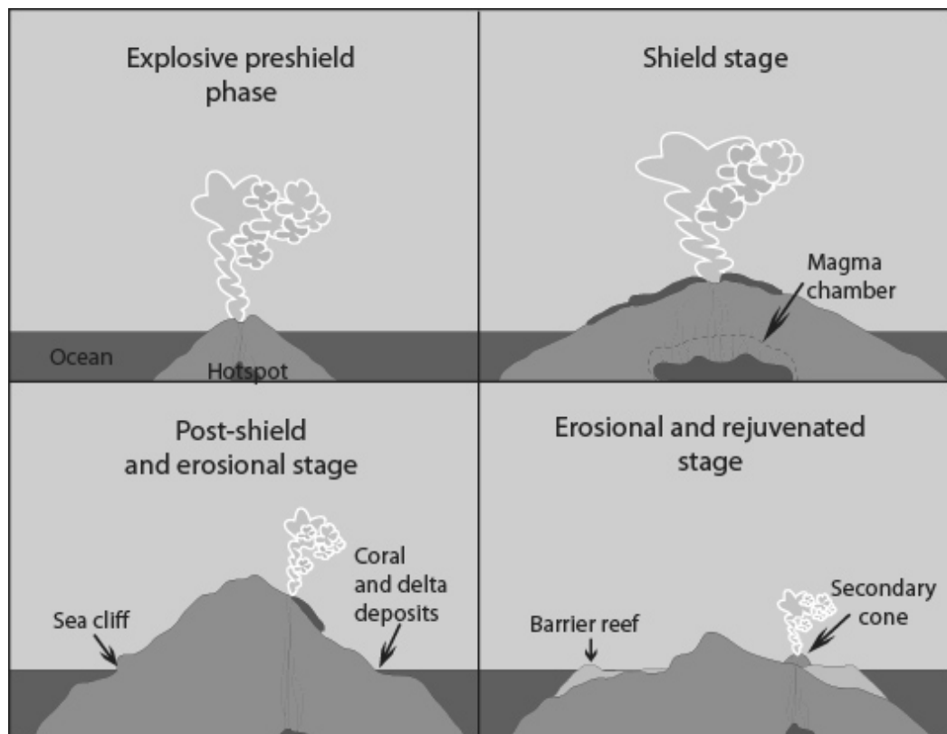
Figure 9. Simplified stages of Hawaiian hotspot volcano growth and erosion. (NPS figure from Thornberry-Ehrlich 2009).
