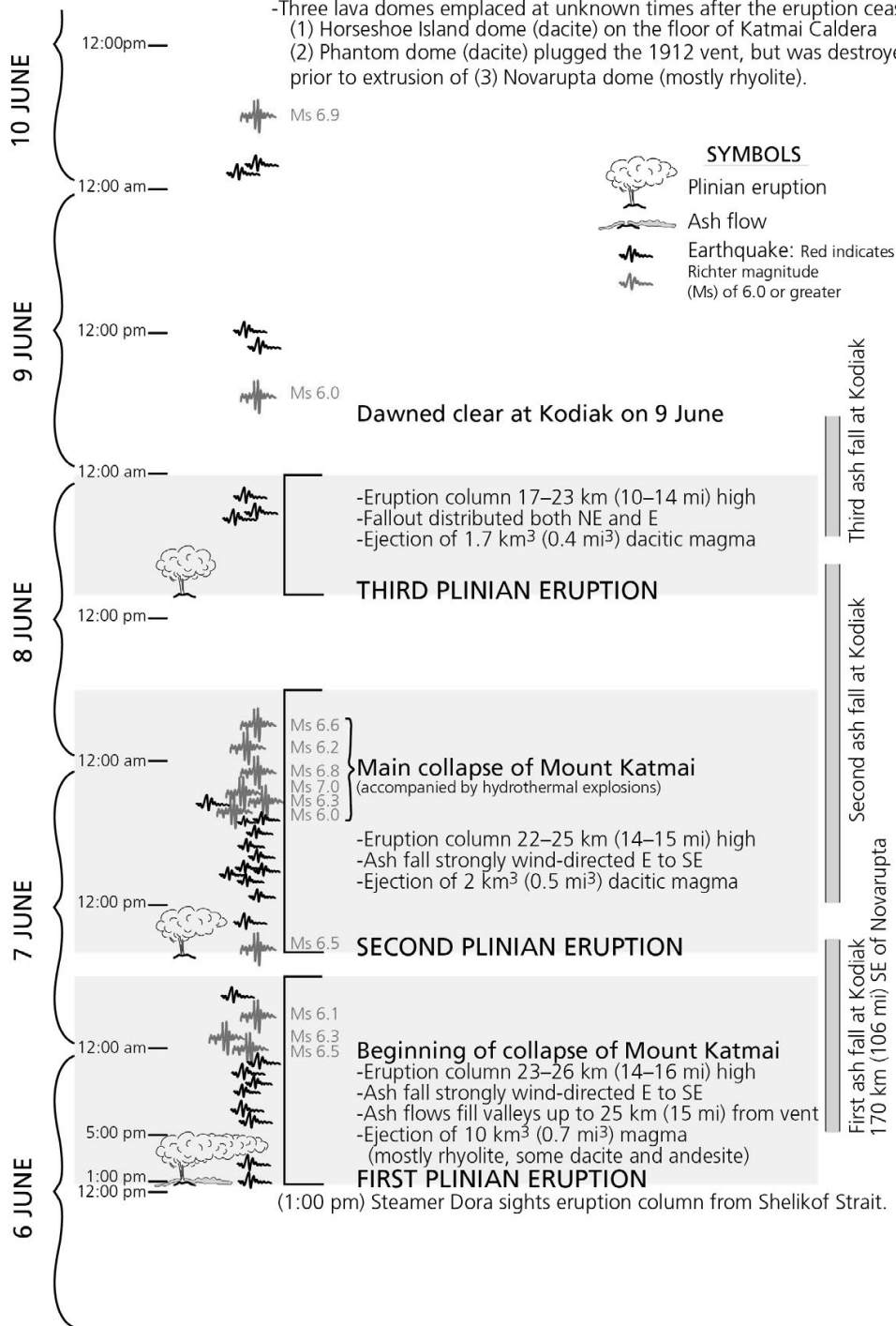
Figure 13. Chronology of the 1912 eruption. There was only one seismograph operating in Alaska in 1912 when the eruption occurred, but many of the earthquakes generated during this eruption were large enough that they were recorded by instruments elsewhere in North America, as well as in Asia, Europe, Hawaii, Japan, and North Africa (NPS figure modified from Hulst and Fierstein 2016).
