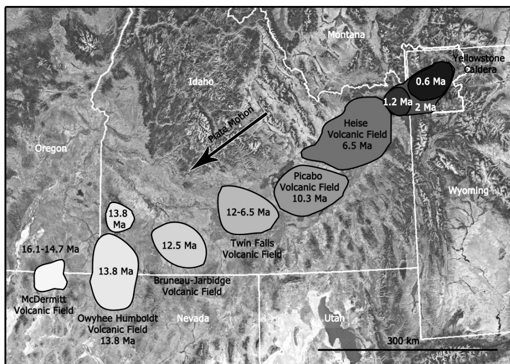
Figure 2: Age progression of the Yellowstone-Snake River Plain trend silicic centers, including the most recent calderas in and near Yellowstone National Park (figure modified from Marcus et al. 2012, and Smith and Siegel 2000).
