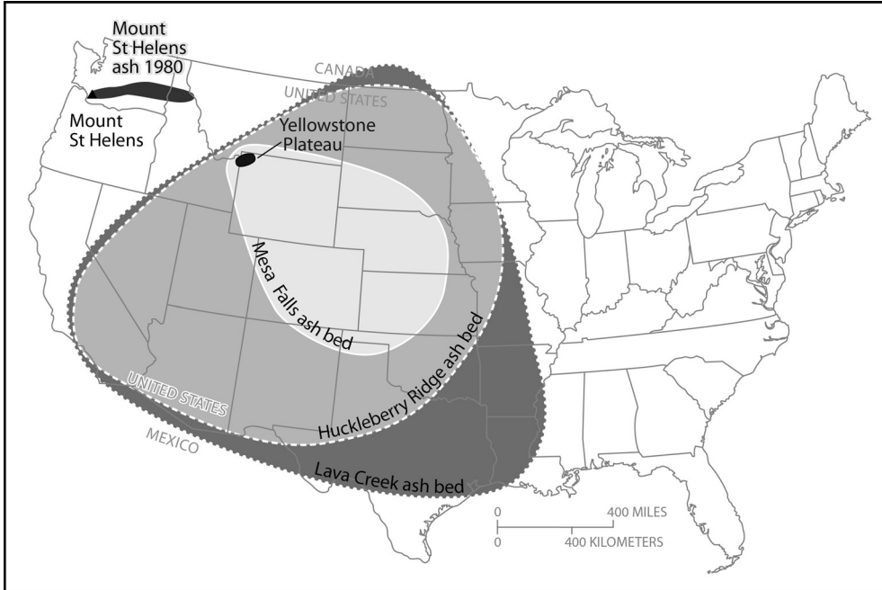
Figure 3: Extent of known ashfall from caldera-forming eruptions at Yellowstone (modified from Lowenstern et al. 2005).
