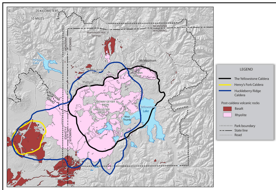
Figure 4: Yellowstone calderas and geography (modified from Lowenstern et al. 2005).
