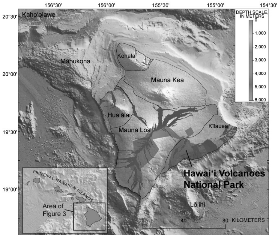
Figure 8. Topography and bathymetry of the Island of Hawai'i. (NPS figure from Thornberry-Ehrlich 2009).
