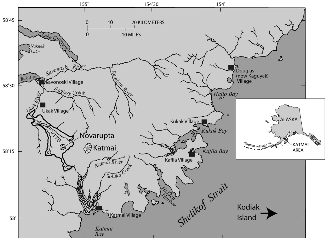
Figure 10: Locations of the populated areas near Katmai in 1912. USGS Alaska Volcano Observatory figure modified from Adleman 2002.
