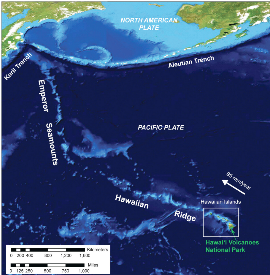
Figure 7. Map of the Hawaiian Ridge – Emperor Seamount Chain. NPS figure from Thornberry-Ehrlich, 2009.
