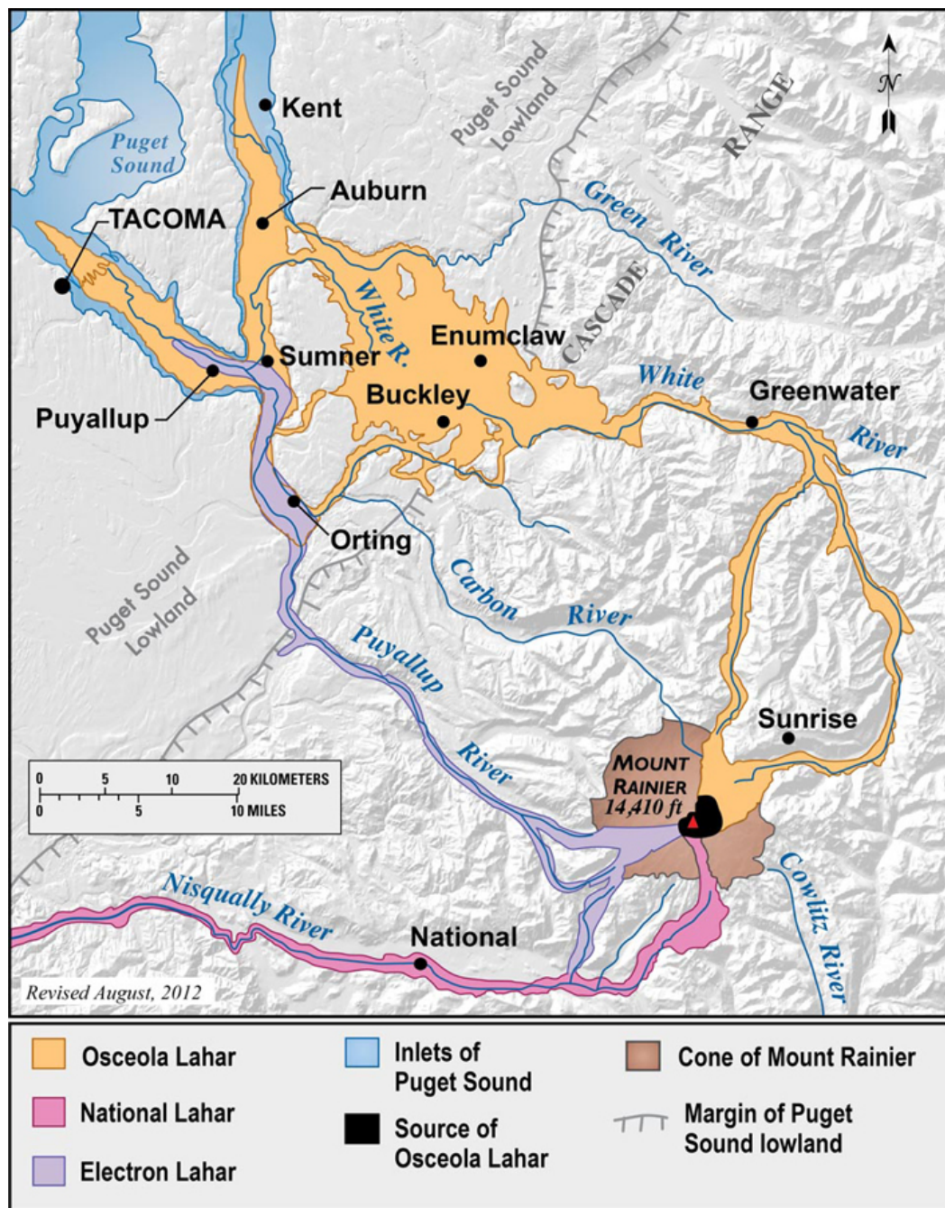
Figure 6. Map showing extents of previous lahars from Mount Rainier. USGS figure modified from Driedger et al. 2005
